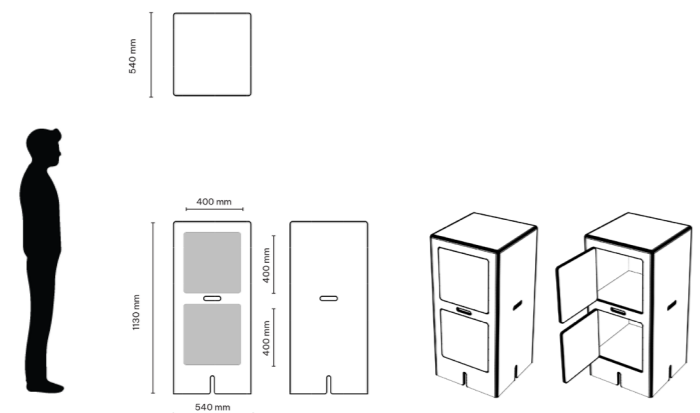
LOCKER H113 2 DOORS
