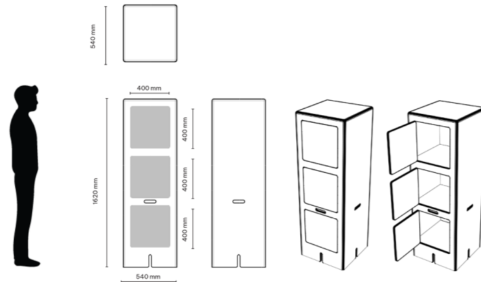
LOCKER H162 3 DOORS
